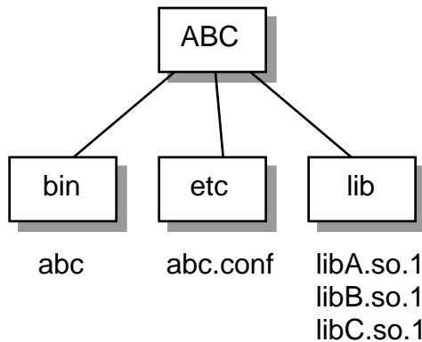
Figure C-1 Unbundled Dependencies
