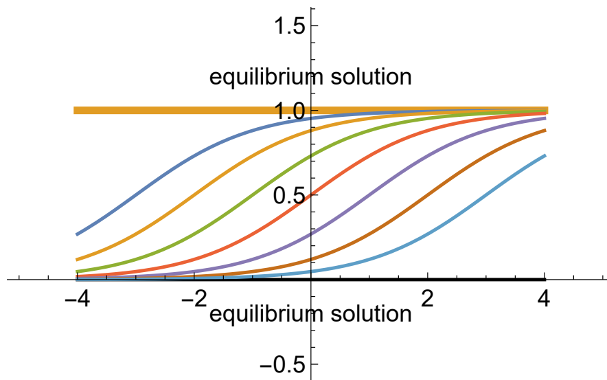
Figure 8: Equilibrium solution envelope with general solution curves
