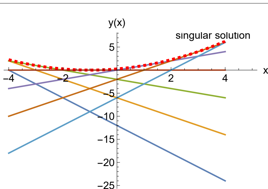
Figure 5: Singular solution envelope with general solution curves
